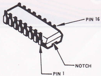
MC14028BCP (Q6002)
